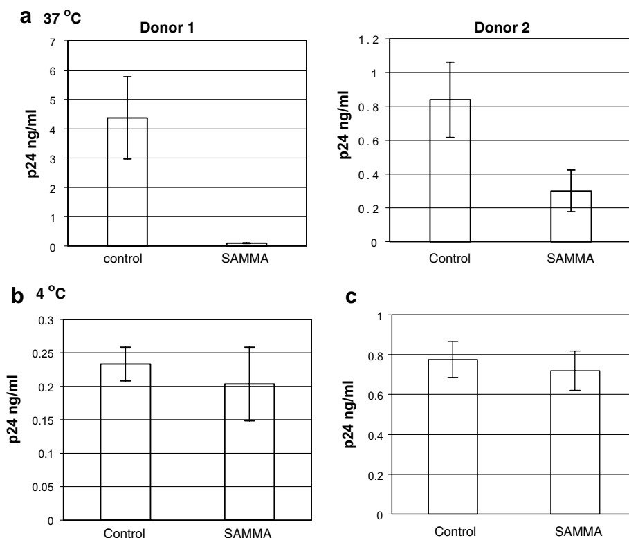
Fig. 4. SAMMA inhibits HIV capture by DCs. MDDC were seeded at 2 \times 10^5 per well in 96-well flat-bottom plates. HIV-1 BaL (3 ng per well) was pre-incubated in the absence (control) or presence of SAMMA for 1 h at 37 °C. DCs were then incubated with virus for 2 h at 37 °C (a) or 4 °C (b) in the absence (control) or presence of the inhibitor. Cells were washed four times to remove unbound virus and SAMMA and lysed with 1% Triton X-100. Cell-associated HIV p24 antigens were measured by p24 ELISA (NCI, Frederick). Data are means \pm SD of duplicated samples. In (a), results from two donors are shown. In (b), results represent two independent experiments from two DC different donors. (c) DCs were treated without (control) or with SAMMA at 100 µg/ml at 37 °C for 1 h and washed four times with PBS followed HIV exposure for 2 h. HIV-exposed DCs were washed and lysed. Cell-associated HIV p24 antigen was measured by ELISA. Results represent two independent experiments from two donors.
