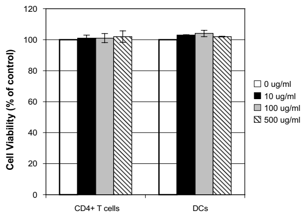
Fig. 3. SAMMA does not cause cytotoxicity in DCs and primary CD4 + T cells. DCs or activated primary CD4 + T cells ( 5 \times 10^4 ) were treated with SAMMA at 10, 100, 500 µg/ml for three days at 37 °C. Cytotoxicity was determined by measuring the number of viable cells by the MTS assay (Promega). MTS substrate was added to cells for 1 h at 37 °C. Data are means \pm SD of triplicated samples and represent two independent experiments.
