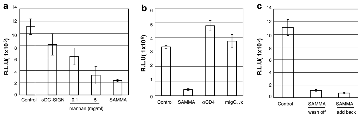
Fig. 2. SAMMA inhibits HIV infection in trans by DCs in a single-round infection assay. (a) MDDCs ( 1 \times 10^6 ) were incubated with SAMMA (100 µg/ml), mannan (0.1 and 5 mg/ml) or anti-DC-SIGN antibody (20 µg/ml, mAb 612 from R&D systems) for 1 h at 37 °C and then exposed to pseudotyped HIV JR-FL luciferase reporter virus for 2 h at 37 °C. Cells were washed four times before co-culturing with HeLa-CD4.CCR5 cells for 48 h. DCs were removed by washing and luciferase activity in relative light unit (RLU) in HeLa cells were measured. (b) DCs were incubated with SAMMA at 100 µg/ml, anti-CD4 antibody (10 µg/ml, Leu3a from BD Biosciences) or an isotype control antibody (mouse IgG 1, κ ) at 37 °C for 1 h followed by exposure to pseudotyped HIV JR-FL luciferase reporter virus for 2 h. DCs were washed and then co-cultured with HeLa-CD4.CCR5 cells for 48 h before measurement of luciferase activity in HeLa cells. (c) DCs were exposed to pseudotyped HIV JR-FL luciferase reporter virus for 2 h at 37 °C and then incubated without or with SAMMA at 100 µg/ml for 1 h at 37 °C. DCs were washed four times with PBS and then co-cultured with HeLa-CD4.CCR5 cells in the absence (wash-off) or presence (add back) of SAMMA for 48 h. Luciferase activity in HeLa cells was measured. Data are means \pm SD of triplicated samples and represent three independent experiments.
