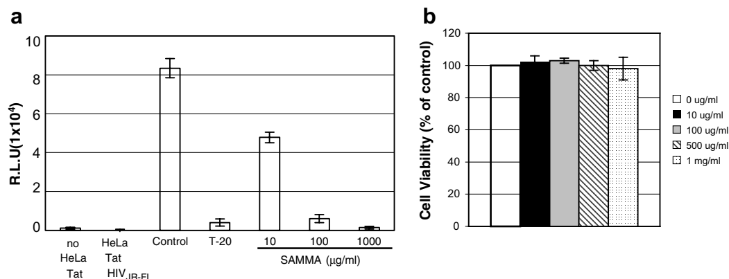
Fig. 5. SAMMA inhibits HIV glycoprotein-mediated cell–cell fusion. HeLa-Tat cells were transfected HIV JR-FL envelope plasmid for 48 h. Cells were then treated with a fusion inhibitor T-20 or SAMMA at 37 °C for 1 h before addition to TZM cells, indicator cells expressing CD4, CXCR4 and CCR5 and containing a luciferase reporter gene driven by HIV LTR. After incubation at 37 °C for 24 h, luciferase activity was measured. Data are means ± SD of duplicated samples and represent three independent experiments. (b) Viability of TZM-bl cells in the presence of SAMMA at various concentrations for 48 h was determined by MTS assay as described in Fig. 3.
