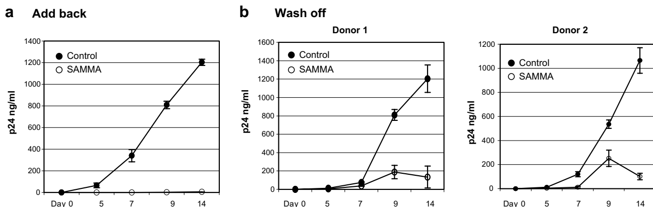
Fig. 1. SAMMA inhibits HIV transmission by DCs. (a) MDDCs ( 1.25\text{--}2 \times 10^5 per well) were exposed to replication-competent R5 virus HIV BaL at MOI of 0.002 in the presence or absence of SAMMA at 100 µg/ml at 37 °C for 2 h. Cells were washed and co-cultured with autologous activated primary CD4 + T cells ( 1 \times 10^6 ) in complete media in the presence or absence of SAMMA at 100 µg/ml. (b) HIV BaL was pre-incubated without (control) or with SAMMA at 100 µg/ml at 37 °C for 1 h followed by addition to DCs ( 2 \times 10^5 ) for 2 h in the absence or presence of the inhibitor. After washing four times with media, DCs ( 1.25 \times 10^5 ) were incubated with activated primary CD4 + T cells ( 1 \times 10^6 ) in the absence of SAMMA. HIV released into media was monitored by measuring the level of HIV p24 antigen at day 0, 5, 7, 9, 14 after infection. Data in (a) are means \pm SD of duplicated samples and represent two independent experiments. In the wash-off setting (panel b), results from two different donors are shown.
